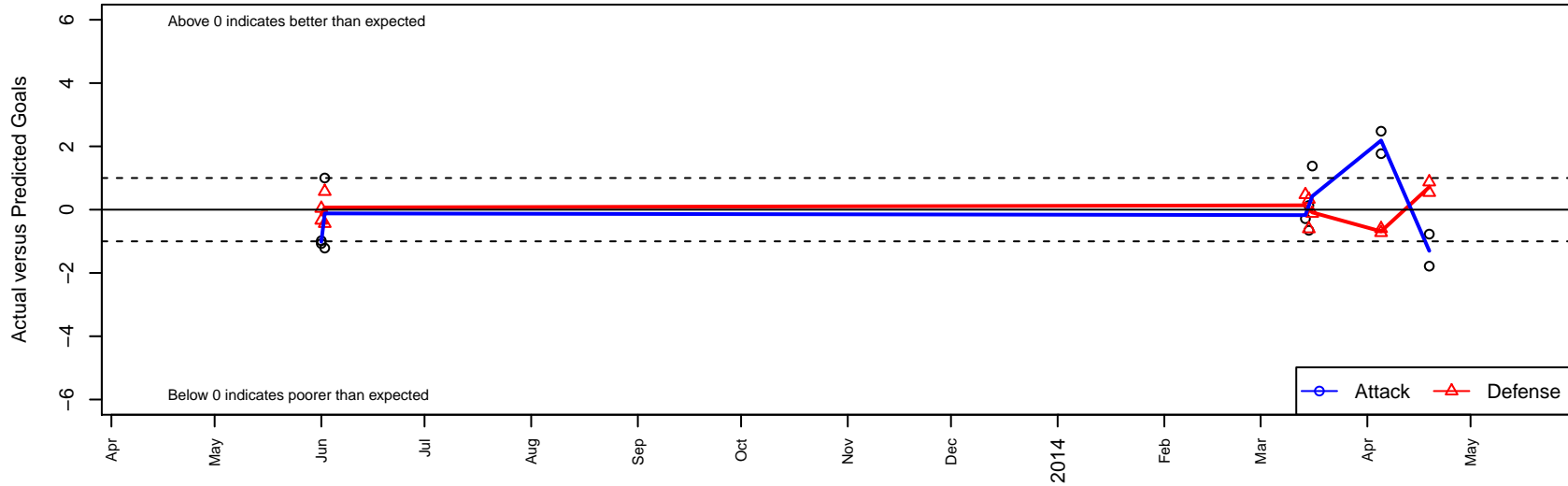
Ballistic SC B96 Dots are actual minus expected GF (blue circles) and GA (red triangles). Blue line is smoothed change in attack strength. Red is smoothed change in defense strength.
